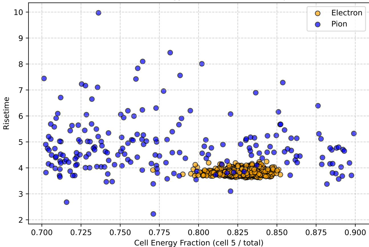
Risetime vs Cell Energy Fraction for 80.0GeV particles
